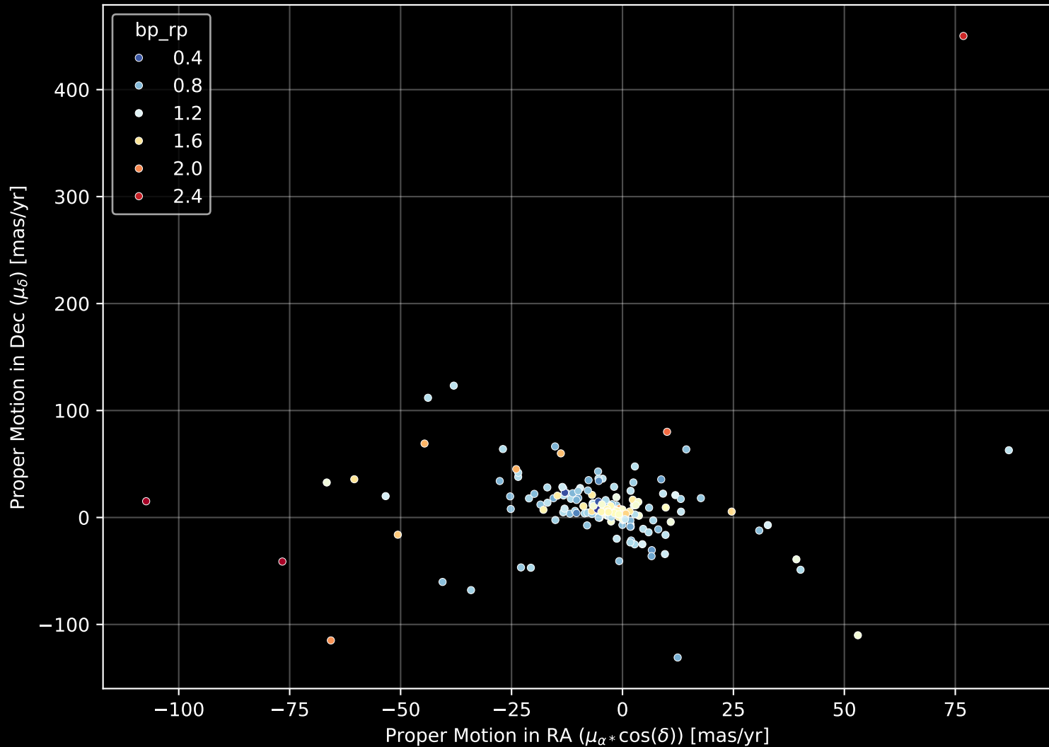
APOGEE DR17 Field: [271-19-O_TESS] Proper Motion Diagram (n= 171)
