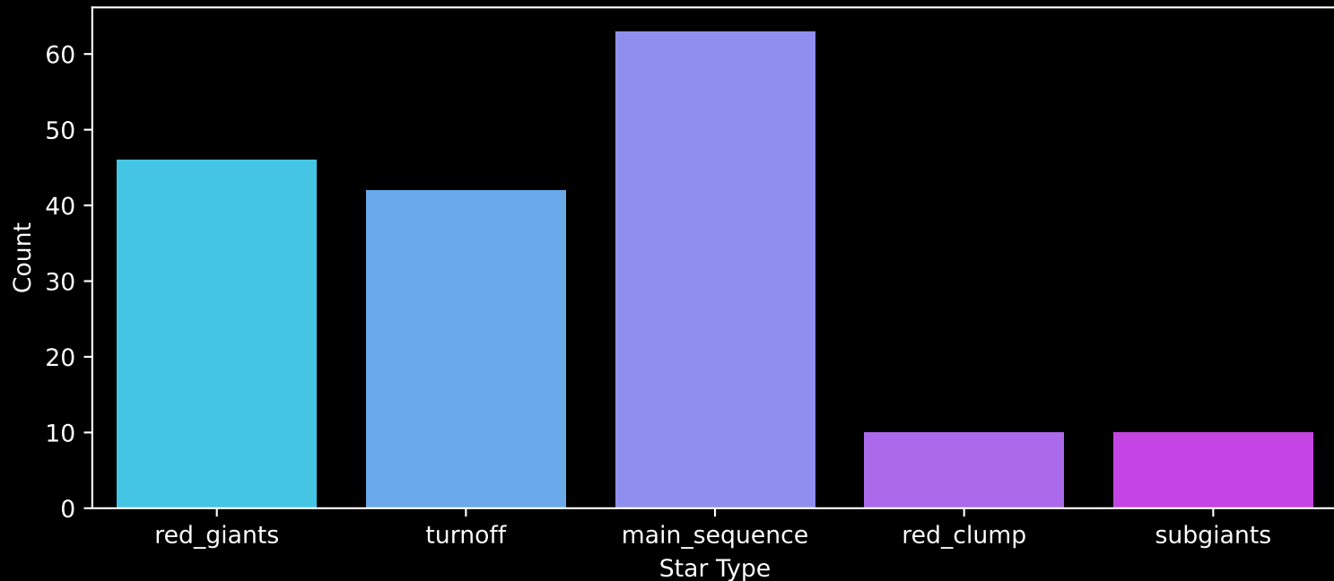
APOGEE DR17 Field: [271-19-O_TESS] Count plot of Star Type
